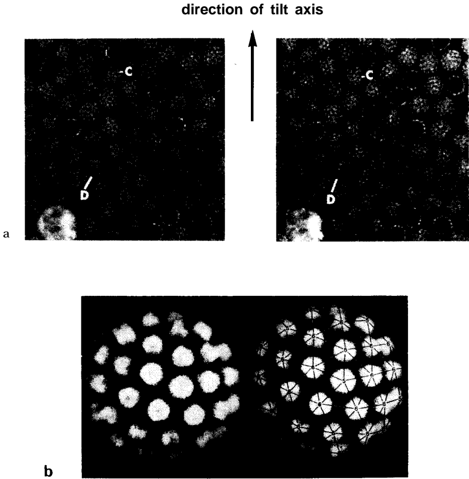
Fig. 10. (a) Electron micrographs of the same field of negatively-stained close-packed particles of human wart virus (HWV) before (i) and after (ii) tilting the specimen grid through an angle close to 18^\circ (73). \times 100,000 .
