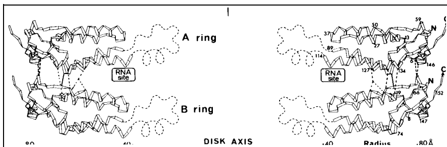
Fig. 4. Section through a disk along its axis reconstructed from the results of X-ray analysis to a resolution of 2.8 \text{ \AA} (15). The ribbons show the path of the polypeptide chain of the protein subunits. Subunits of the two rings can be seen touching over a small area toward the outside of the disk but opening up into the "jaws" toward the centre. The dashed lines at low radius indicate schematically the mobile portion of the protein in the disk, extending in from near the RYA binding site to the edge of the central hole
