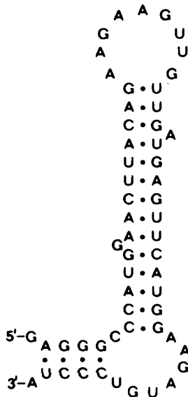
Fig. 6. Postulated secondary structure of the RNA in the nucleation region (24). This gives a weakly bonded double-helical stem and a loop at the top probably the actual origin of assembly. The sequence at and near the top contains a repeating motif of three bases having G in the middle position and A, or U in the outer positions.
