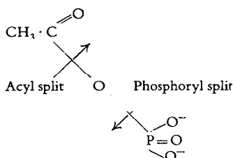
Fig. 3. Acetyl phosphate as acetyl and phosphoryl donor.
