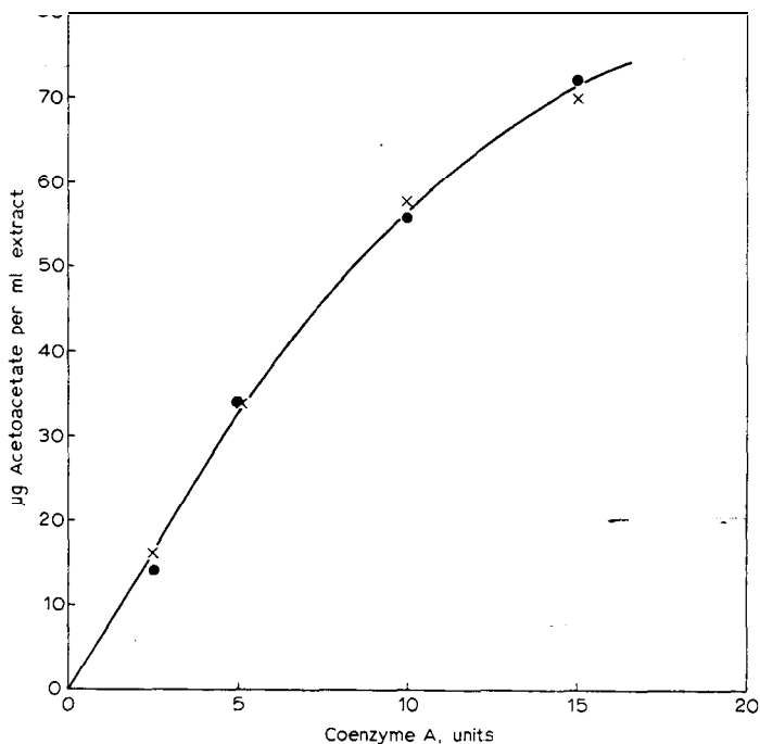
Fig. 8. Coenzyme A dependence of acetoacetate formation from acetate + ATP with ammonium sulfate pigeon-liver fraction.
