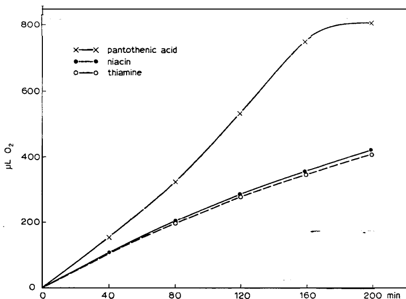
Fig. 5a. Effect of coenzyme A on acetate oxidation in yeast. Pantothenate-deficient yeast was preincubated in glucose-phosphate medium with 50 \mu g of pantothenate, 100 \mu g of thiamine, and 100 \mu g of niacin in separate flasks; 5.6 mg of dry weight of each suspension were added to individual Warburg vessels. Total fluid volume 3.0 ml of 0.06 M \text{KH}_2\text{PO}_4 and 0.01 M acetic acid; temperature 37°; gas phase air.
