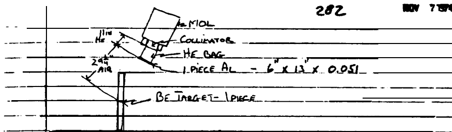
Fig. 13a. Aluminium foil arrangement in front of magnet M_0 in our new experiment to determine the e/\pi ratio. The converter was used to determine the electron background yield.
