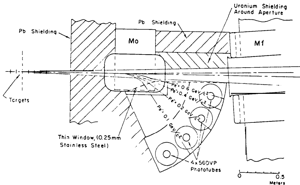
a. Side view of magnet M_0 which bends the various low-energy trajectories ( P_e ) of e^+ into C_B .
