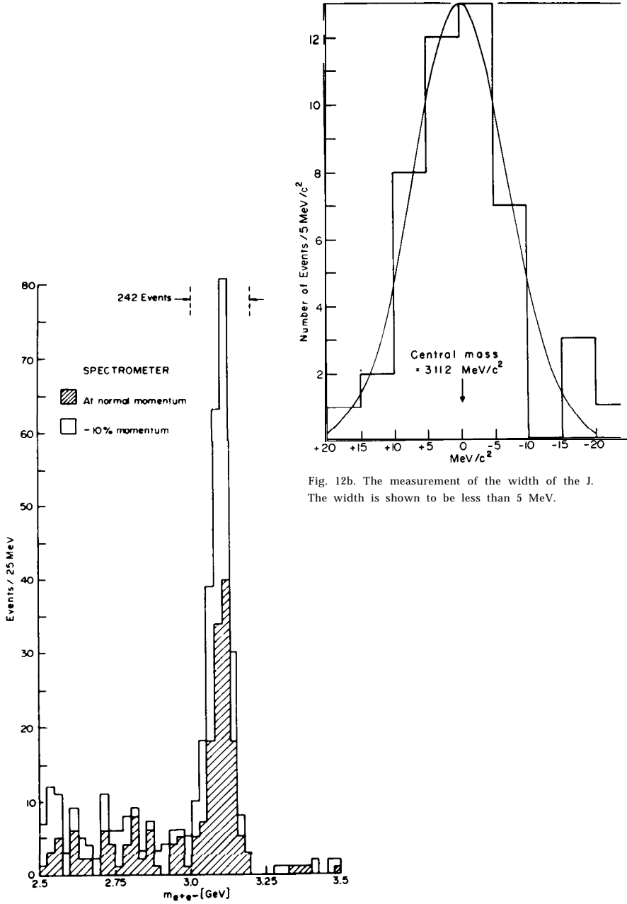
Fig. 12a Mass spectrum for events in the mass range 2.5 < m_{ee} < 3.5 GeV/c. The shaded events correspond to those taken at the normal magnet setting, while the unshaded ones correspond to the spectrometer magnet setting at -10% lower than normal value.
