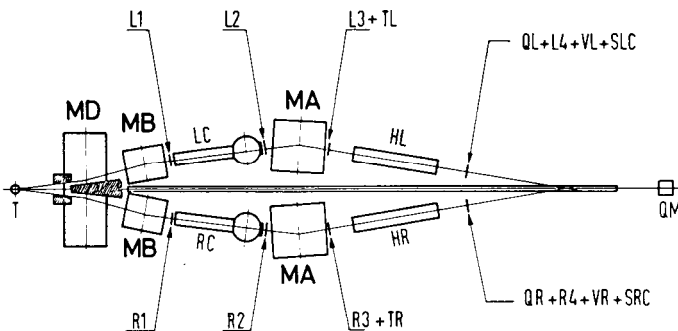
Fig. 1a. Plan view of the spectrometer. MD, MA, RIB are dipole magnets; L1, . . . . L4, and R1, . . . . R4, are triggering counters; LC, RC, and HL, HR are large-aperture threshold Čerenkov counters; SLC, SRC are shower counters; and TL, QL, VL, and TR, QR, VR are hodoscops. QM is a quantameter.
