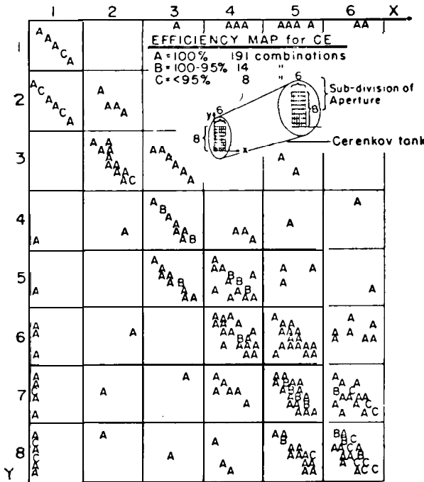
Fig. 11 a. Mapping of the efficiency of the C_e counter over its whole phase space. The letters on the plot refer to efficiencies measured for trajectories between the corresponding points marked on the grid at each end of the counter.
