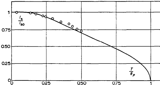
Fig.12. Temperature dependence of the spontaneous magnetization of manganese antimonide Mn_2Sb (experimental points and curve calculated with the molecular field coefficients deduced from the study of susceptibility).
