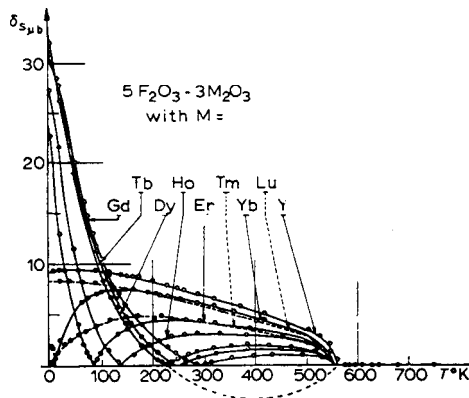
Fig.19. Temperature dependence of the spontaneous magnetization of a series of garnet ferrites. In particular, it will be noted how the compensation point varies with the atomic number of the rare earth.
