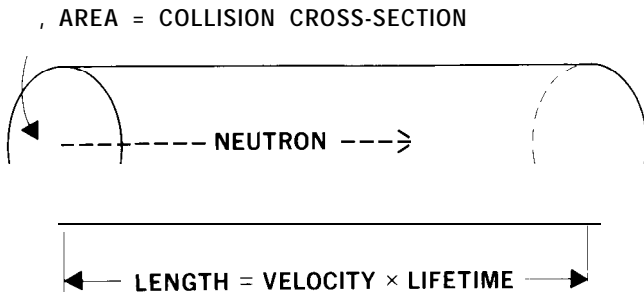
Fig. 3 Gamow's Sample Cylinder ; The volume swept out by a neutron in the early universe. The length of the cylinder is the product of the neutron's thermal velocity (at 10^9\text{K} ) and its decay time. The cross-sectional area is the neutron-proton collision cross-section for deuteron formation. The fraction of neutrons forming deuterons is equal to the probability that the cylinder contains a proton.
