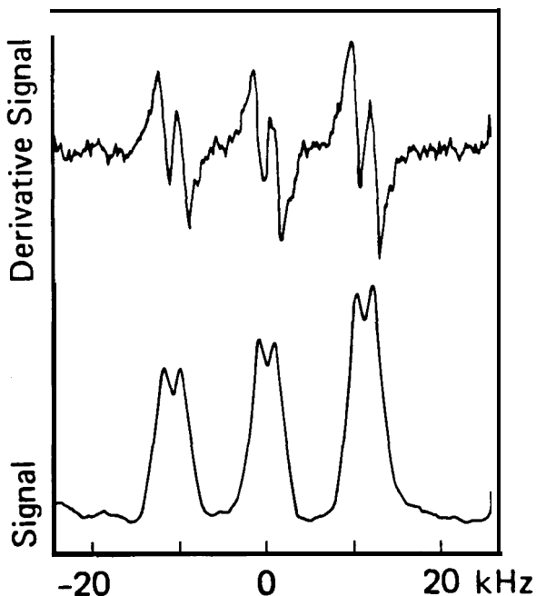
Fig. 5. High resolution ( < 1 kHz) saturation spectroscopy of a ^{12}\text{C H}_\alpha spectral line near 3.39 \mu\text{m} wavelength. Each of the three hyperfine components is split into a doublet from the optical recoil effect. The upper curve is the experimental derivative trace (after reference 36).
