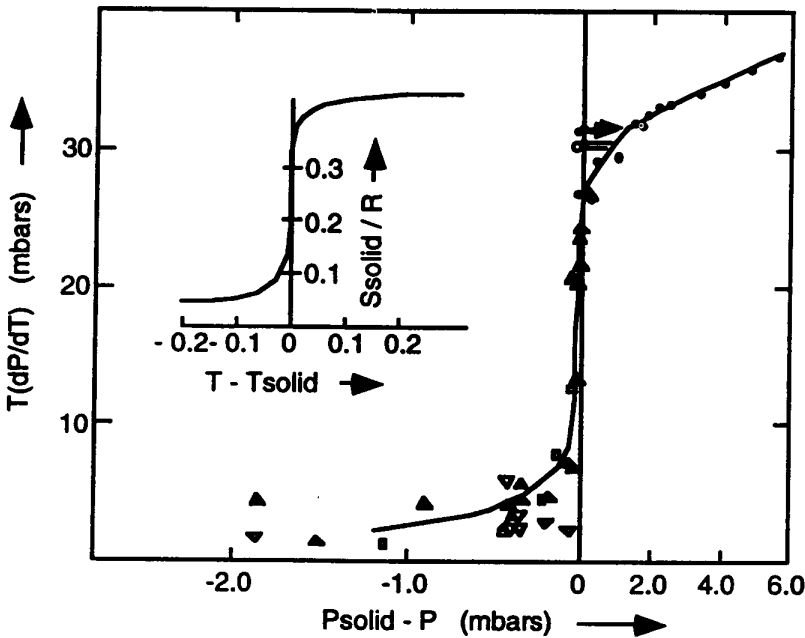
Figure 13. The entropy decrease at the nuclear magnetic phase transition of solid ^3\text{He} . The entropy versus temperature data were calculated from the measurements of T(dP/dP) versus pressure.
