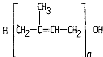
Fig. 3. Polyprenols.
