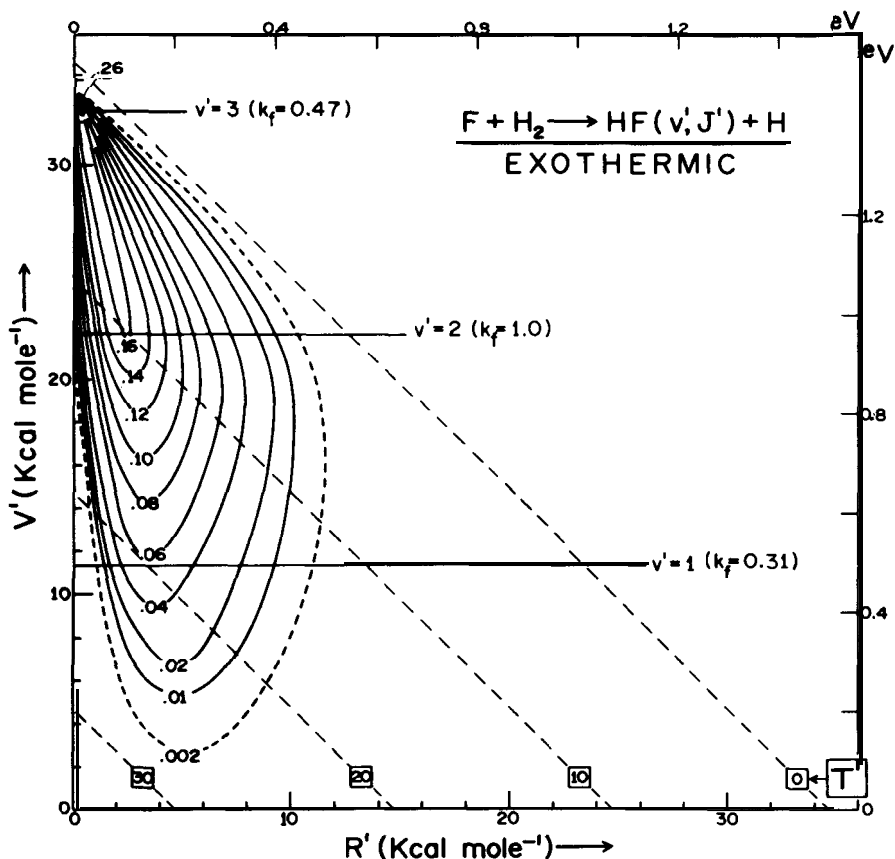
Figure 8. Triangle plot for F+H_2 \rightarrow HF+H (see caption to fig. 6). E'_{tot} = 34.7 kcal/mole for this reaction. From J.C. Polanyi and K.B. Woodall, J. Chem. Phys. 57, 1574 (1972).
