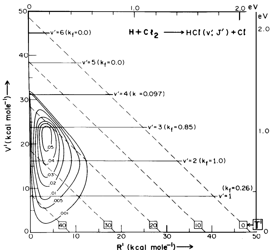
Figure 6. 'Triangle plot' for \text{H} + \text{Cl}_2 \rightarrow \text{HCl}(\nu', J') + \text{Cl} reaction showing the distribution of vibrational, rotational, and translational energy as contours of equal detailed rate constant k(V', R', T') . The ordinate is product vibrational energy, and the abscissa is the product rotational energy. Since the total available energy is approximately constant ( E_{\text{avail}} = 48.4 kcal/mole), translational energy, T' , given by the broken diagonal lines, increases to 48.4 kcal/mole at V' = 0, R' = 0 . The rate constant k_{\text{f}} = k(\nu') = \sum_j k(\nu', J'_j) ; the subscript f denotes the 'forward', exothermic, direction. Contours have been normalized to k(\nu') = 1.00 where \nu' is the most-populated vibrational level. From K.G. Anlauf et al., J. Chem. Phys. 57, 1561 (1972).
