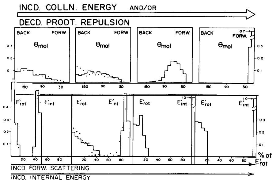
Figure 18. Effect of repulsive energy release on product angular distribution (top row) and energy distribution (bottom row; E'_{tot} is product rotational excitation and E'_{int} is vibration plus rotation). The solid lines show the results of 3D (three-dimensional) DIPR model calculations (masses K+Br_2 , energy-release E'_{int} = 53 kcal/mole). The total product repulsion used in the DIPR model calculations was decreased in four stages, from left to right in the figure, simulating decreased % R , implying increased % A . According to the DIPR model this is mathematically equivalent to increasing the reagent collision energy, hence the dual label of the arrow at the top. The consequences of these changes are summarized, qualitatively, by the arrows at the foot of the figure. The dots record the distributions obtained from 3D trajectories on potential-energy hypersurfaces with comparable partitioning of the energy-release. Adapted from P.J. Kuntz et al., J. Chem. Phys. 50, 4623 (1969).
