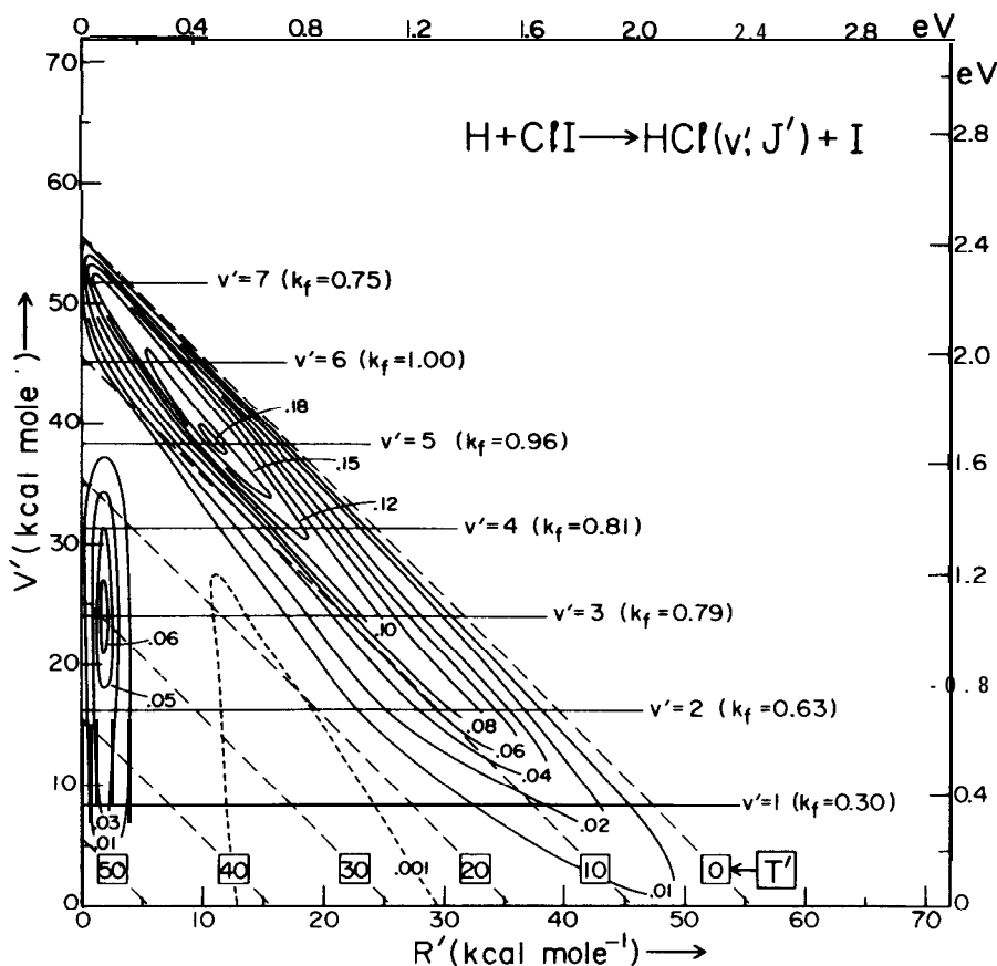
Figure 12. Triangle plot for the reaction \text{H}+\text{ClI} at 300K showing bimodality (18 % of the HCl is in the low -J' mode, 82% in the high -J' ). From M.A. Nazar, J.C. Polanyi, and W.J. Skrlac, Chem. Phys. Letts. 29, 473 (1974). See also J.C. Polanyi and W.J. Skrlac, Chem. Phys. 23, 167 (1977).
