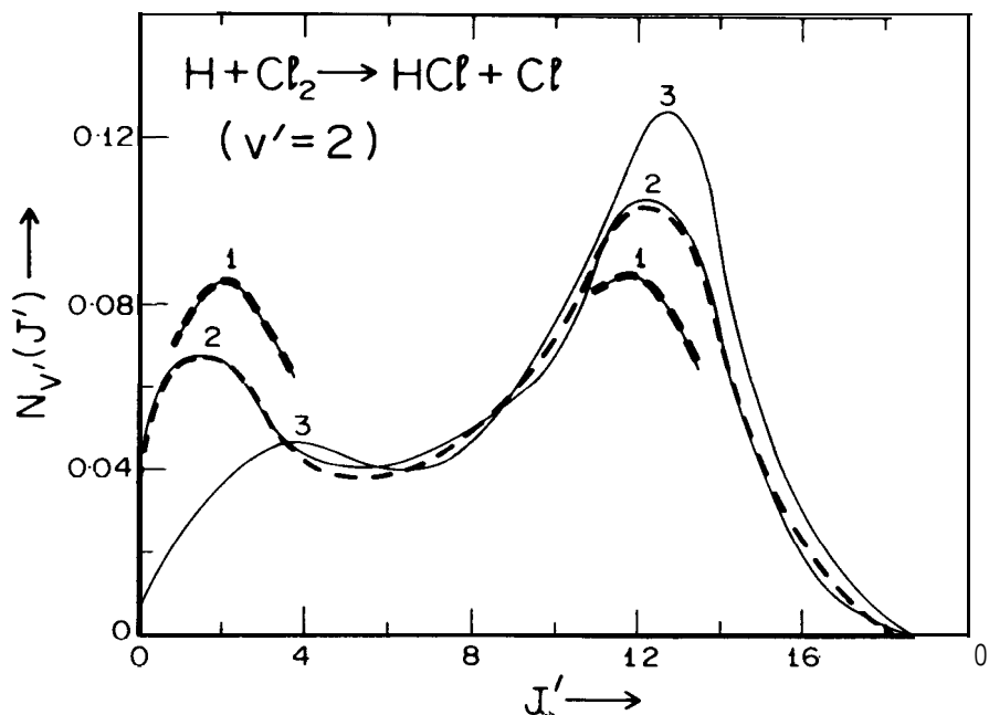
Figure 5. Solid lines record the decreasing contribution of the peak at low J' to the observed rotational distribution (for \text{H} + \text{Cl}_2 \rightarrow \text{HCl} + \text{Cl} , v' = 2 ) as the pressure in the beam-crossing region is decreased (in the sequence 3 \rightarrow 2 \rightarrow 1 ) in an A.R. vessel. The broken lines superimposed on the solid lines give relaxed distributions computed from 3. Based on fig. 1 of J.C. Polanyi and K.B. Woodall, J. Chem. Phys. 56, 1563 (1972).
