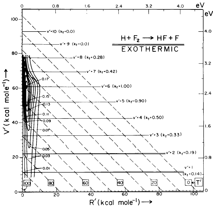
Figure 7. Triangle plot for \text{H} + \text{F}_2 \rightarrow \text{HF} + \text{F} (see caption to fig. 6). E'_0 = 102 kcal/mole for this reaction. From J.C. Polanyi and J.J. Sloan, J. Chem. Phys. 57, 4988 (1972).
