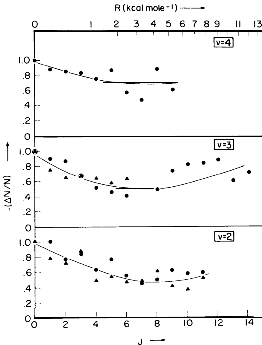
Figure 30. Fractional depletions of individual J states of v = 2-4 in a CD study of the endothermic reaction \text{HF}^\dagger + \text{Na} . From B.A. Blackwell et al., Chem. Phys. 30, 299 (1978).
