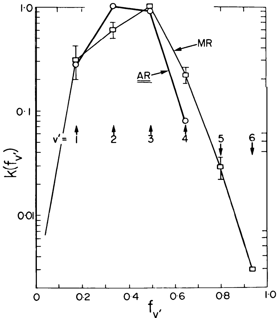
Figure 3. Semi-logarithmic plot of the probability that a fraction f_{v'} of the energy in the products of the reaction \text{H}+\text{Cl}_2 \rightarrow \text{HCl}+\text{Cl} enters vibration in the newly-formed bond. The data were obtained independently by the MR and AR methods, as indicated. The vibrational quantum states v' = 1-6 correspond to the values of f_{v'} indicated by arrows across the centre of the figure. From K.G. Anlauf et al., Disc. Faraday Soc. 44, 183 (1967).
