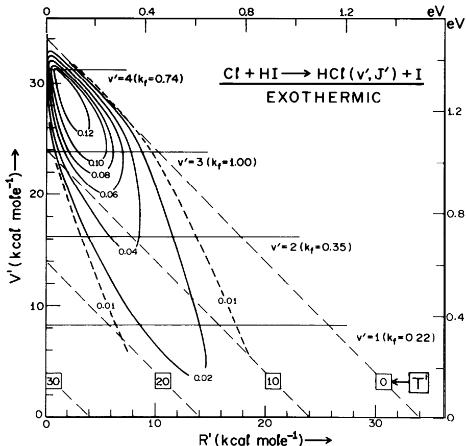
Figure 9. Triangle plot for \text{Cl} + \text{HI} + \text{HCl} + \text{I} . See caption to fig. 7. E'_{\text{in}} = 34 kcal/mole. From D.H. Maylotte et al., J. Chem. Phys. 57, 1547 (1972).
