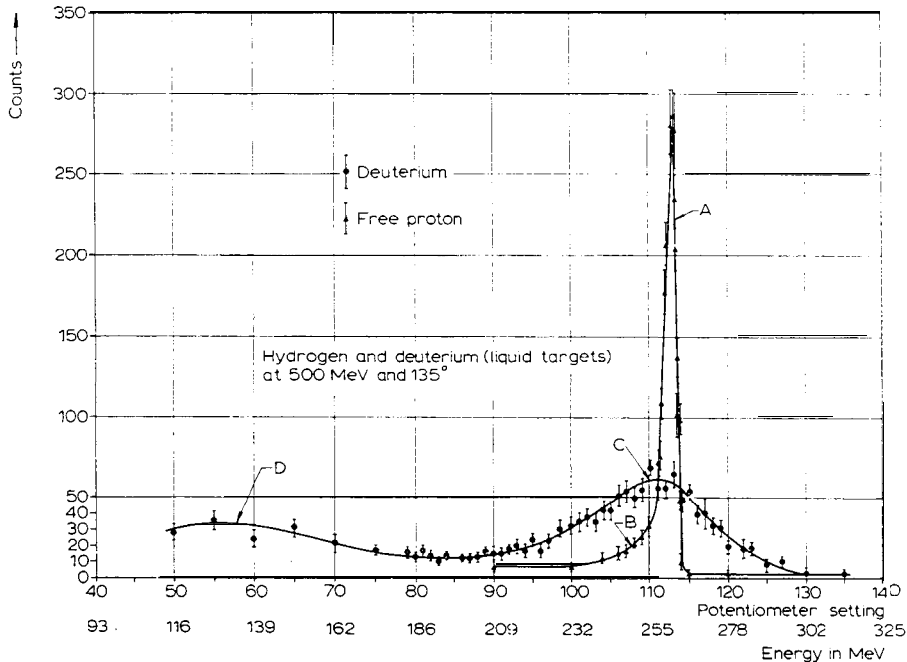
Fig. 11 The experimental comparison of the scattering from the moving proton and neutron in the deuteron (Curve C) and the scattering associated with free protons (Curve A) 18 . Region B shows the bremsstrahlung tail of the proton curve. At D are electrons which have been scattered after producing pions in deuterium and also other low-energy electrons. From the scattering data near C the form factors of the neutron can be obtained. The proton peak is used for comparison measurements. No correction has been applied in the figure for the different densities of liquid deuterium and liquid hydrogen.
