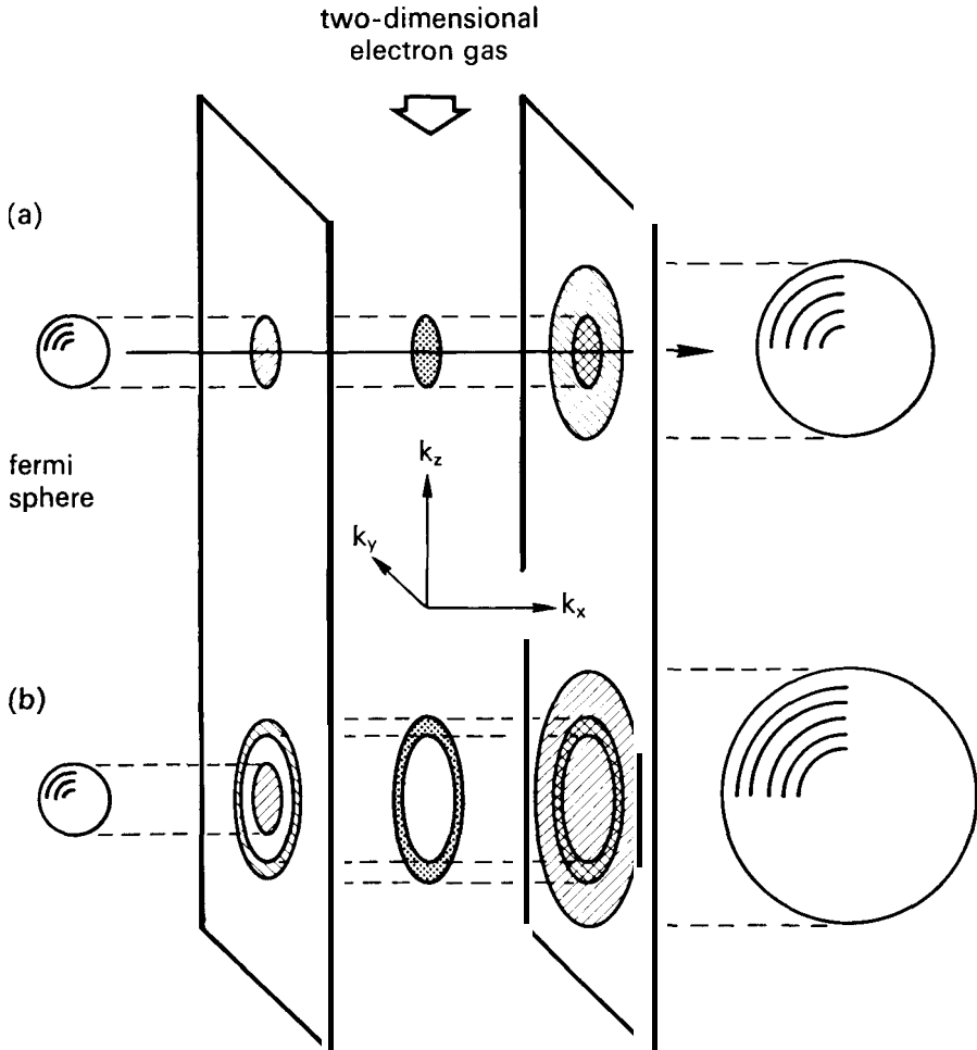
Fig. 12. Construction of shadows of energy surfaces on two k_x - k_z planes corresponding to two barriers.
