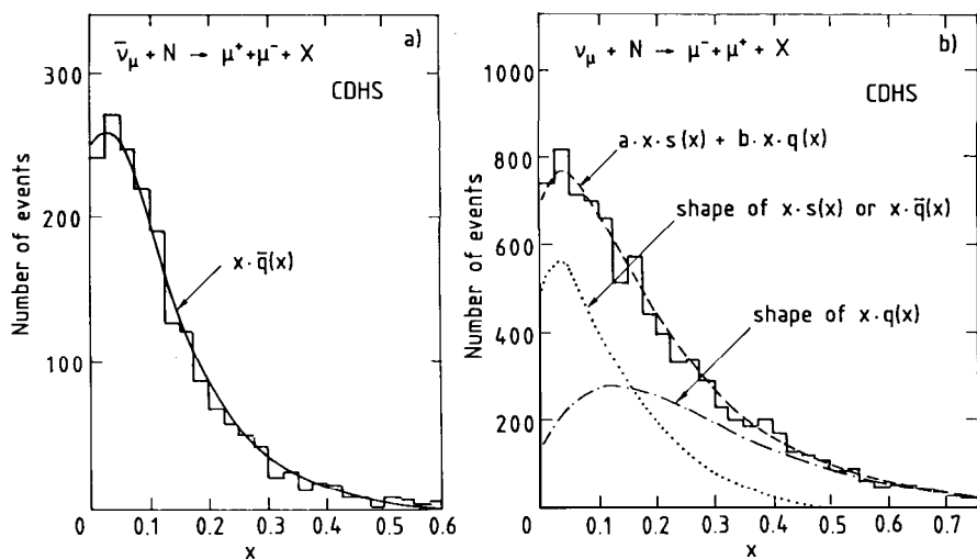
Figure 21 The x -distributions of opposite-sign dimuon events. a) For antineutrinos. The dominant process is \bar{\nu} + s \rightarrow \mu^+ + \bar{c} . The observed x -distribution is therefore that of the strange sea in the nucleon.
