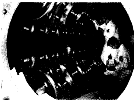
Figure 4 Preparation of the interior of the 13 m bubble chamber Gargamelle, later to be filled with Freon. It is with this detector that the neutral currents were discovered.
