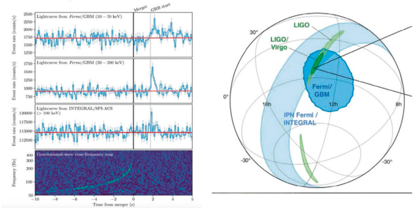
Figure 15. Fermi short gamma ray burst signal observed 1.7 sec after gravitational wave signal in the same region of the sky.
