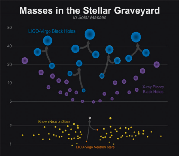
Figure 9. Masses of observed black hole mergers in LIGO.
