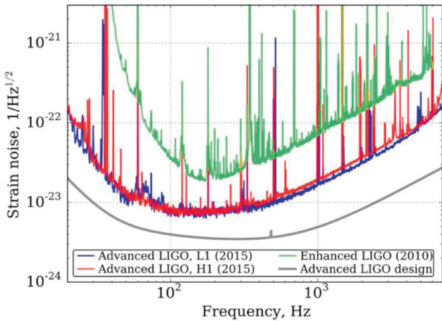
Figure 4. Advanced LIGO Sensitivity Goal.
