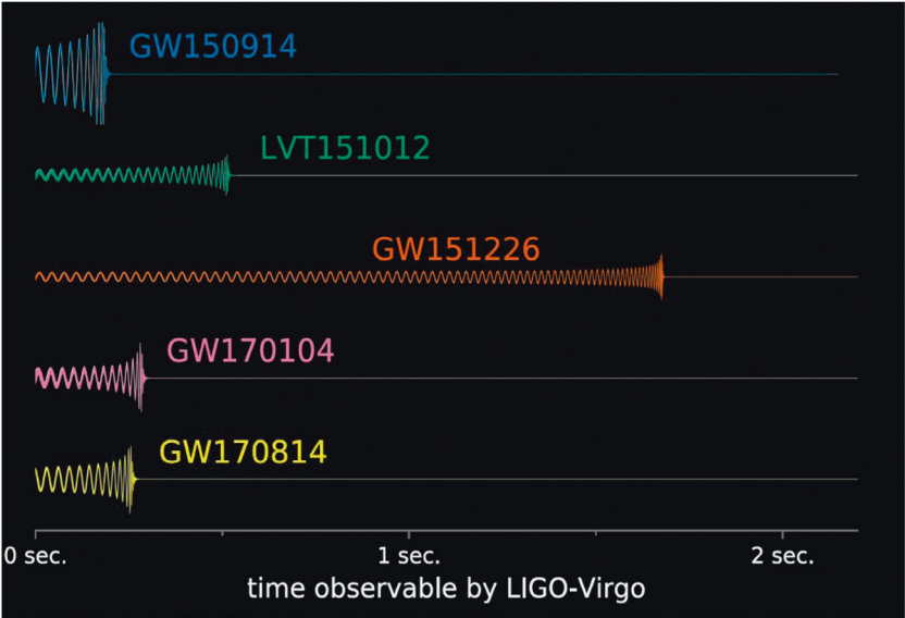
Figure 8. Event characteristics of reported black hole mergers in LIGO.
