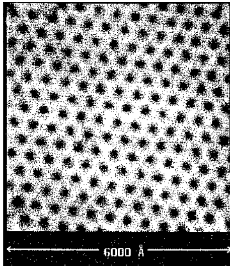
Figure 6. Vortices in NbSe 2 defined by scanning tunneling microscopy (STM).
