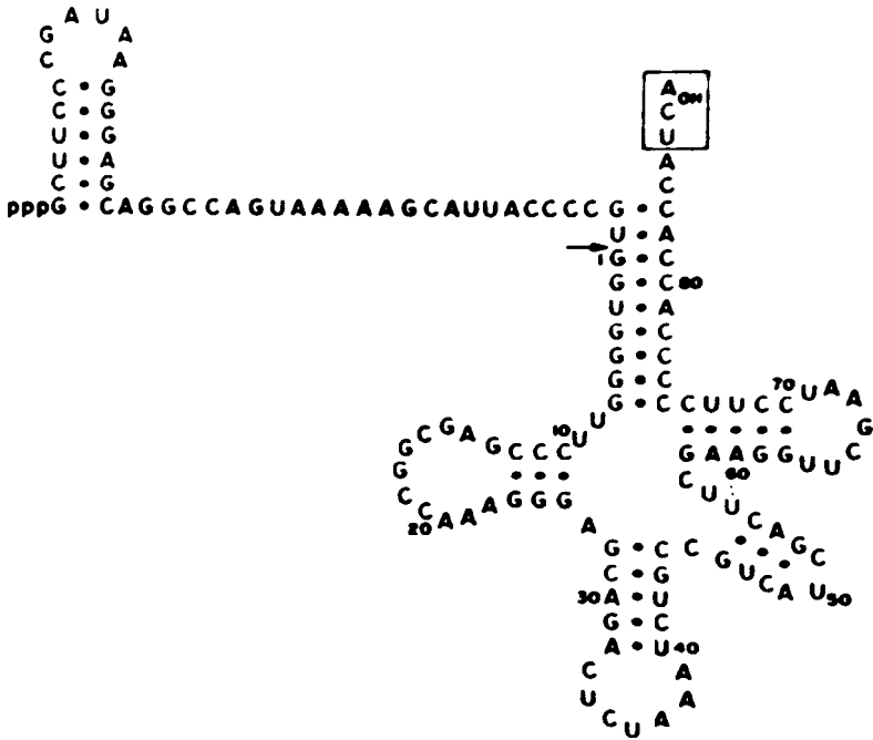
Figure 4. Nucleotide sequence of the precursor to tRNA Tyr su3 + . The arrow pointing toward the sequence indicates the site of cleavage by RNase P on the 5' side of nucleotide 1 of the mature tRNA sequence. The boxed nucleotides are extra nucleotides at the 3' terminus (after Altman and Smith, 1971).
