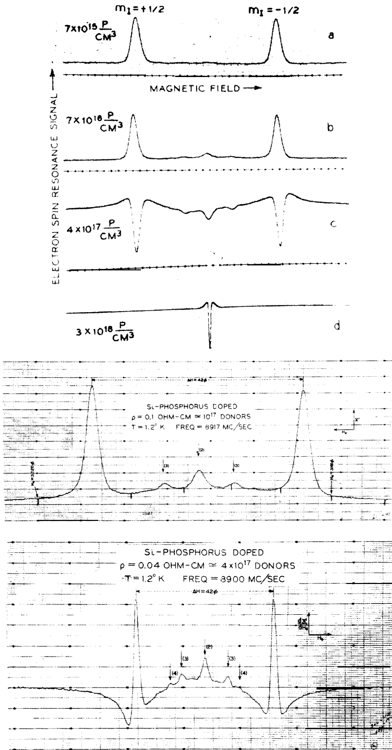
Fig. 10. a) Hyperfine structures of donor EPR at increasing donor (P) concentrations the Mott-Anderson metal-insulator transition. b) Example of well-developed cluster lines.
