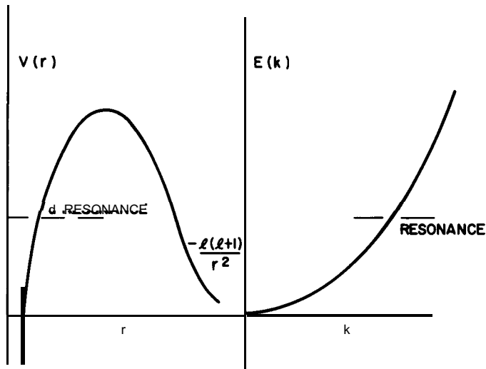
Fig. 4. d -Resonance due to tunneling through the centrifugal barrier.
