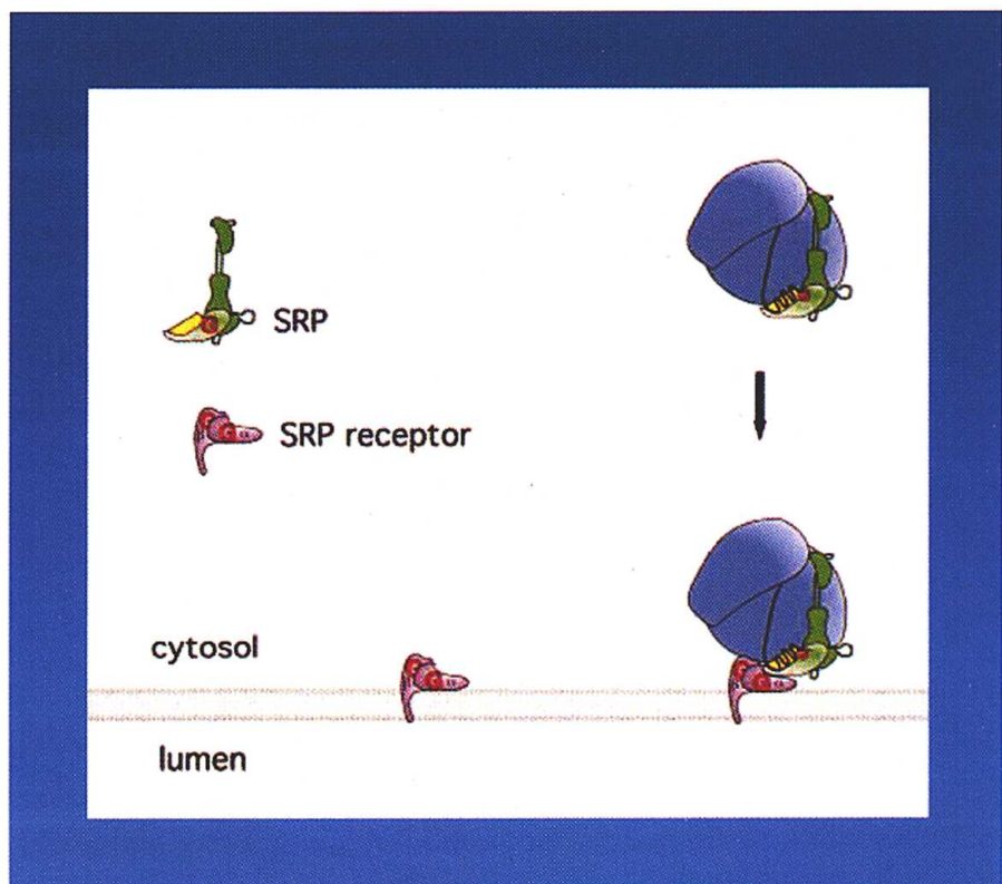
Figure 20. The ribosome/nascent chain/SRP complex binds to the SRP receptor in the ER.
