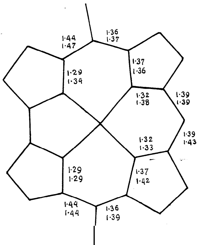
Fig. 9. Interatomic distances (below) found from \sigma_6 for cobyric acid compared with those suggested for a system containing six resonating double bonds.
