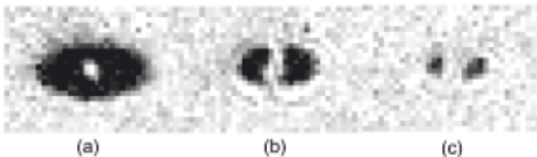
Figure 4. Absorption images of atom clouds trapped in the optically plugged trap. Cloud (a) is already colder than was attainable without the "plug" (Ar ion laser beam). Cloud (b) shows the break-up of the cloud into two "pockets" in the two minima of the potential. The size of cloud (c) reached the optical resolution of the imaging system ( \leq 10 \mu\text{m} ) still absorbing 90 % of the probe light. This sets an upper bound on temperature ( \leq 10 \mu\text{K} ) and a lower bound on density ( 5 \times 10^{12} \text{cm}^{-3} ).
