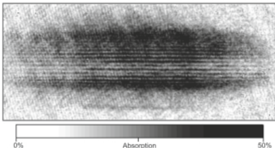
Figure 15. Interference pattern of two expanding condensates observed after 40 ms time-of-flight. The width of the absorption image is 1.1 mm. The interference fringes have a spacing of 15\text{ }\mu\text{m} and are strong evidence for the long-range coherence of Bose-Einstein condensates.
