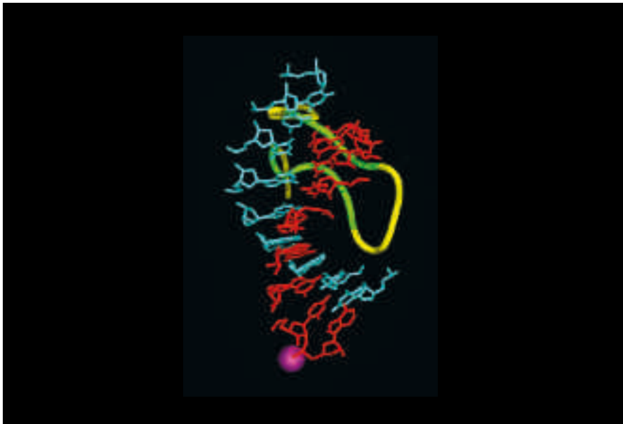
Figure 14. Superposition of the DNA-hybrid helix from an RNA polymerase II transcribing complex (Fig. 6) and the B finger from an RNA polymerase II-TFIIB complex (Fig. 13). Conserved region of the B finger is green.
