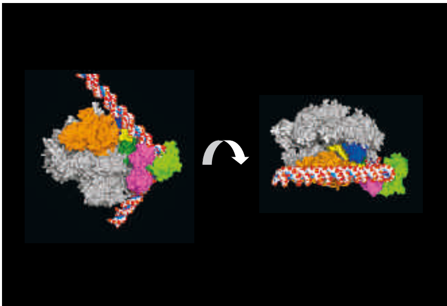
Figure 15. Model of an RNA polymerase II-TBP-TFIIB-DNA complex. The structure of the C-terminal region of TFIIB (pink) complexed with TBP (green) and TATA-box containing DNA (red/white/blue atomic model) was docked to the structure of the pol II-TFIIB complex (as shown in Fig. 13). The views in the left and right panels are related by a 90° rotation about an axis between them, as indicated by the curved arrow. The direction of view in the right panel is the same as that in Fig. 13.
