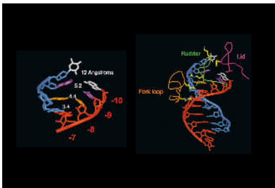
Figure 12. Release of RNA transcript from DNA-RNA hybrid revealed in the structure of an RNA polymerase II transcribing complex. The upstream end of the DNA-RNA hybrid helix, 7-10 residues from the active center, is shown on the left, with distances between the DNA and RNA bases indicated. The entire DNA-RNA hybrid helix is shown on the right, along with protein loops involved in helix melting (rudder and lid) and stabilization (fork loop).
