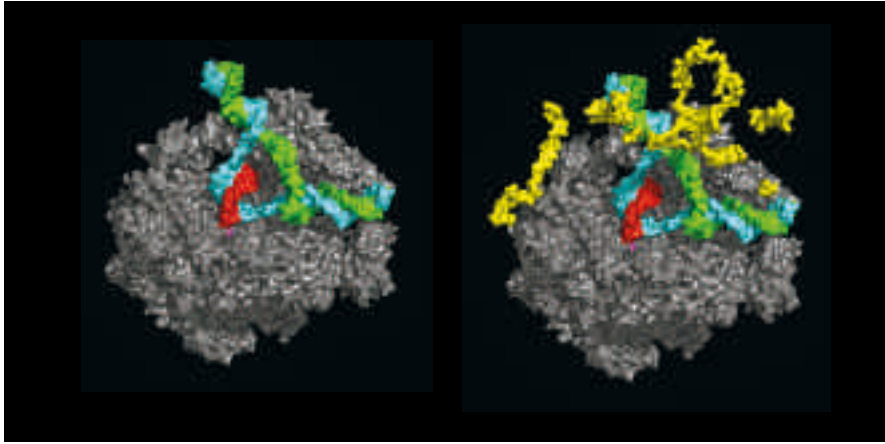
Figure 16. Structure of an RNA polymerase II transcribing complex with the central subunit of TFIIF (work in progress of Guillermo Calero). Pol II and the nucleic acids only are shown on the left, while the structure including the TFIIF subunit (known as Tfg2, in yellow) is shown on the right. Direction of view and color scheme as in Fig. 6.
