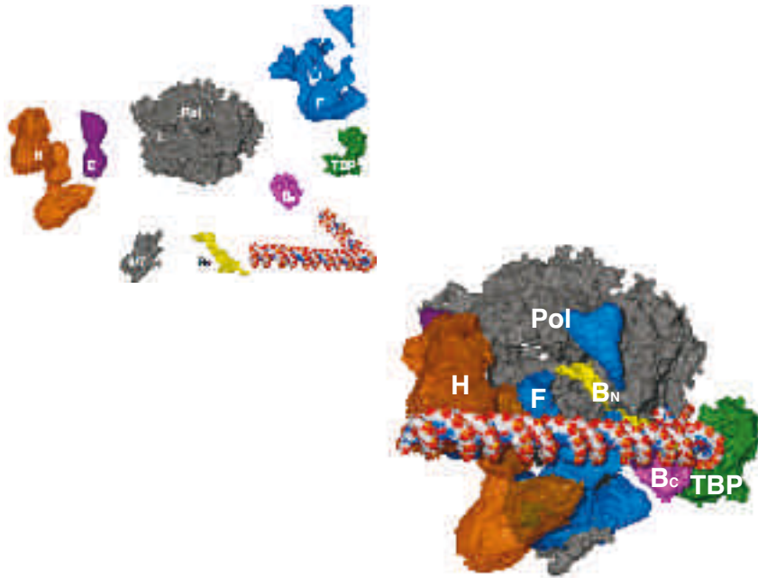
Figure 17. Model of an RNA polymerase II pre-initiation complex. Structures shown at the upper left were assembled in the complex shown at the lower right. Direction of view as in Figs. 5 and 13. “4/7” indicates pol II subunits Rpb4 and Rpb7, which were omitted from the original structure (Fig. 5).
