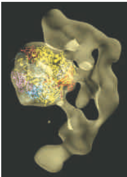
Figure 18. Cryo-EM structure of an RNA polymerase II-Mediator complex. The pol II structure was docked in the central density, and is shown in a similar direction of view and color scheme as Fig. 5.
