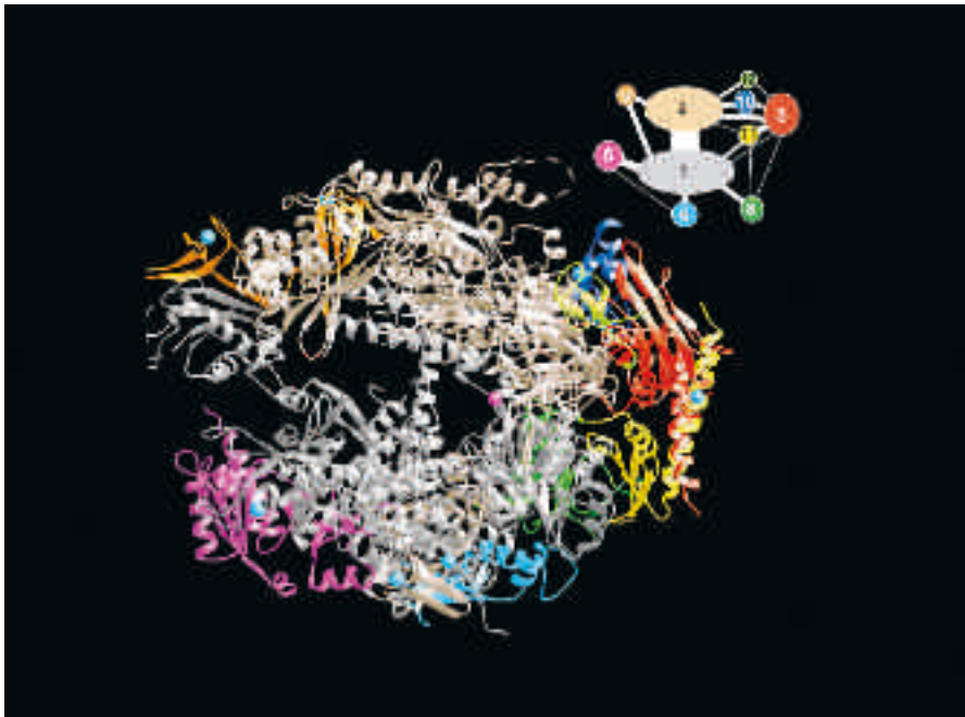
Figure 5. Structure of RNA polymerase II at 2.8 Å resolution. The protein is shown in ribbon representation, with a color code to the various subunits and interaction diagram at the upper right. A Mg ion at the active center is depicted as a pink sphere.
