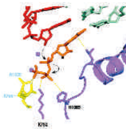
Figure 10. The trigger loop couples NTP recognition to phosphodiester bond formation. Color scheme as in Fig. 8, with side chains of Rpb2 Arg1020 and Rpb2 Arg766 in yellow. Contacts responsible for alignment, and for the contact of histidine 1085 with the NTP that promotes catalysis, are indicated by dashed yellow lines. Nucleophilic attack and phosphoanhydride bond breakage are indicated by black arrows.
