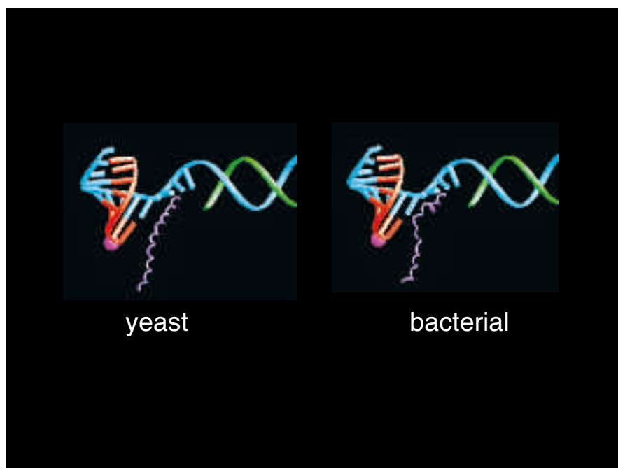
Figure 11. Straight and bent states of the bridge helix in RNA polymerase II and bacterial RNA polymerase structures, proposed to underlie nucleic acid translocation during transcription. Color code as in Fig. 6 except with bridge helix in purple.
