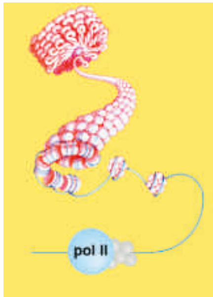
Figure 1. The nucleosome, fundamental particle of the eukaryote chromosome. Schematic shows the coiling of DNA around a set of eight histones in the nucleosome, the further coiling in condensed (transcriptionally inactive) chromatin, and uncoiling for interaction with the RNA polymerase II (pol II) transcription machinery.
