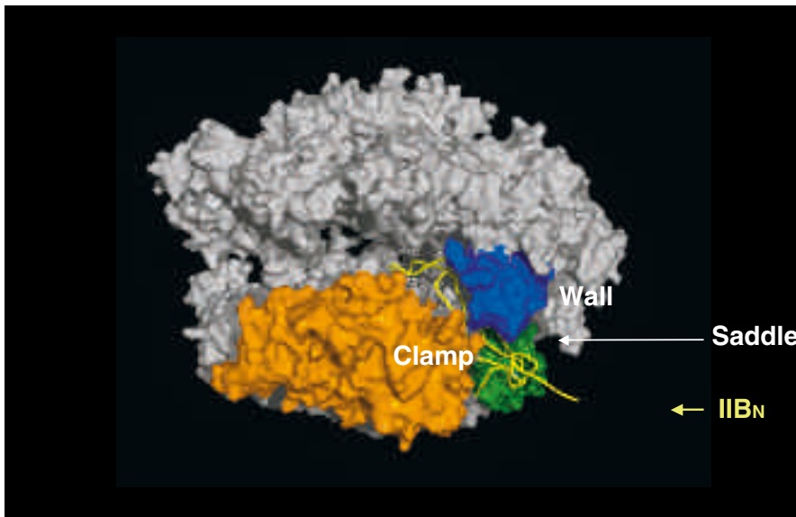
Figure 13. Structure of an RNA polymerase II-TFIIB complex. A surface representation of pol II is shown, with the clamp and wall as in Fig. 6, a polypeptide chain trace of the amino terminal region of TFIIB, designated IIB N , in yellow, and the region of the pol II surface interacting with IIB N in green.
