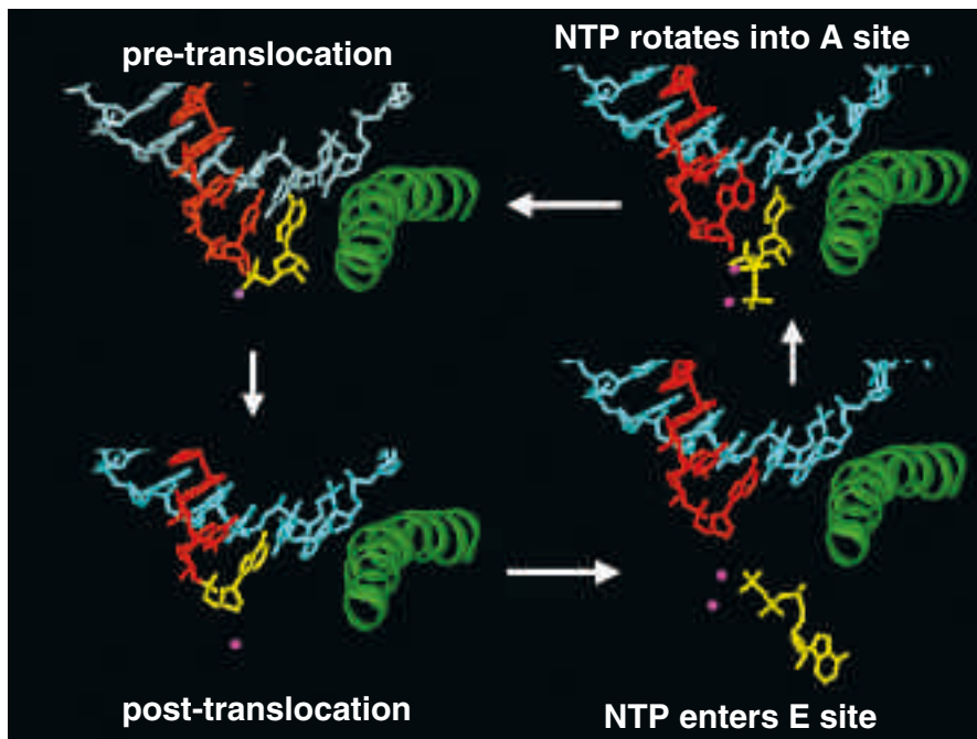
Figure 7. A cycle of nucleotide addition by RNA polymerase II. At the upper left, the structure from Fig. 6 is shown, omitting all but the DNA and RNA near the active center and the bridge helix. The ribonucleotide in the active center, just added to the RNA chain, is yellow. At the lower left is the structure after translocation of DNA and RNA across the pol II surface. At the upper right is the structure with NTP, matched for pairing to the coding base in the template strand, in the addition (A) site.
