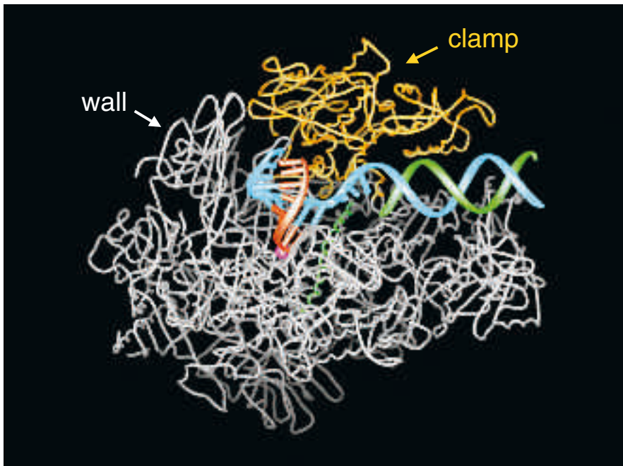
Figure 6. Structure of RNA polymerase II in the act of gene transcription at near atomic resolution. The polypeptide chain is shown in white, orange (mobile “clamp”), and green (bridge helix connecting the two largest subunits). Backbone models of the nucleic acids are shown in blue (template DNA strand), green (nontemplate DNA strand), and red (RNA).
