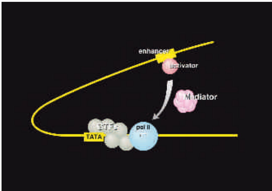
Figure 2. Mediator of transcriptional regulation. Schematic shows the transduction of regulatory information from a gene activator protein bound to an enhancer DNA element to the pol II transcription machinery at a promoter.
