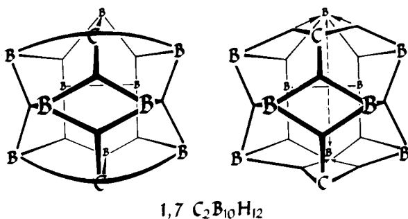
Fig. 32. A situation parallel to that of Fig. 31 may occur in 1,7\text{-C}_2\text{B}_{10}\text{H}_{12} , where the Boys localization (right side) shows fractional bonds. The open three-center bond description may be found by the Edmiston-Ruedenberg procedure, if and when the calculations can be made.
