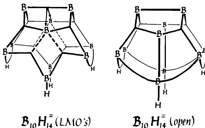
Fig. 38. A relationship similar to that in B_{20}H_{16} occurs in B_{10}H_{14}^- . The preferred localized orbital structure is shown on the left side, while the open three-center bond structure without donation is an oversimplified valence structure.
