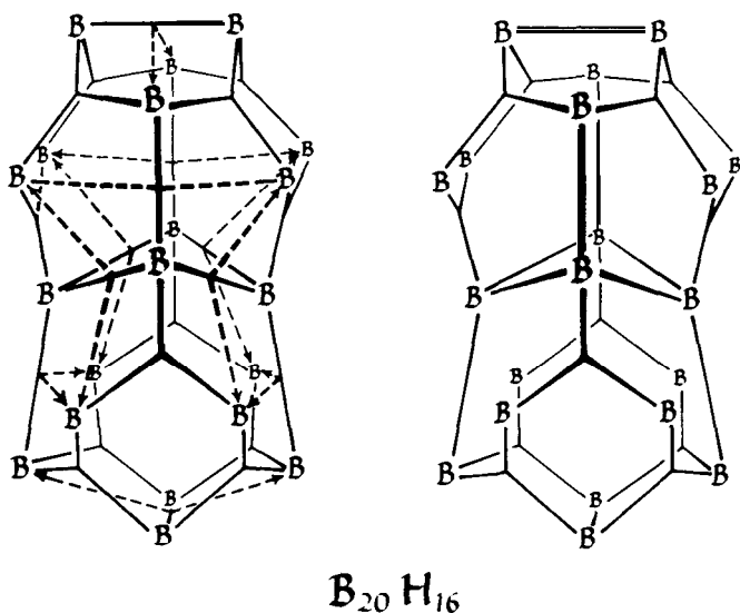
Fig. 37. Donation and non-donation localized orbitals are shown for B_{20}H_{16} in which the four borons nearest the equatorial belt have no terminal hydrogens. Boron atoms B_4B_{16} , inclusive, are particularly electron deficient, and receive substantial donation from single bonds. Each of these eight boron atoms has only two framework bonds in the figure at the right.
