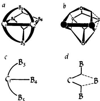
Fig. 31. In 1,2\text{-C}_2\text{B}_4\text{H}_6 the Edmiston-Ruedenberg localization yields open three-center bonds at carbon, while the Boys localization gives fractional three-center bonds. The latter procedure gives greater emphasis to separation of orbital centroids when they are on the same atom.
