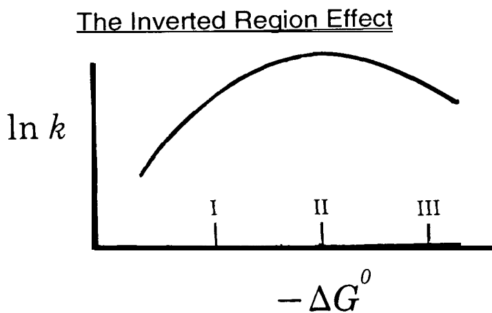
Figure 7. Plot of \ln k , vs -\Delta G^\circ . Points I and III are in the normal and inverted regions, respectively, while point II, where \ln k , is a maximum, occurs at -\Delta G^\circ = \lambda (Marcus and Siddarth, ref. 2).
