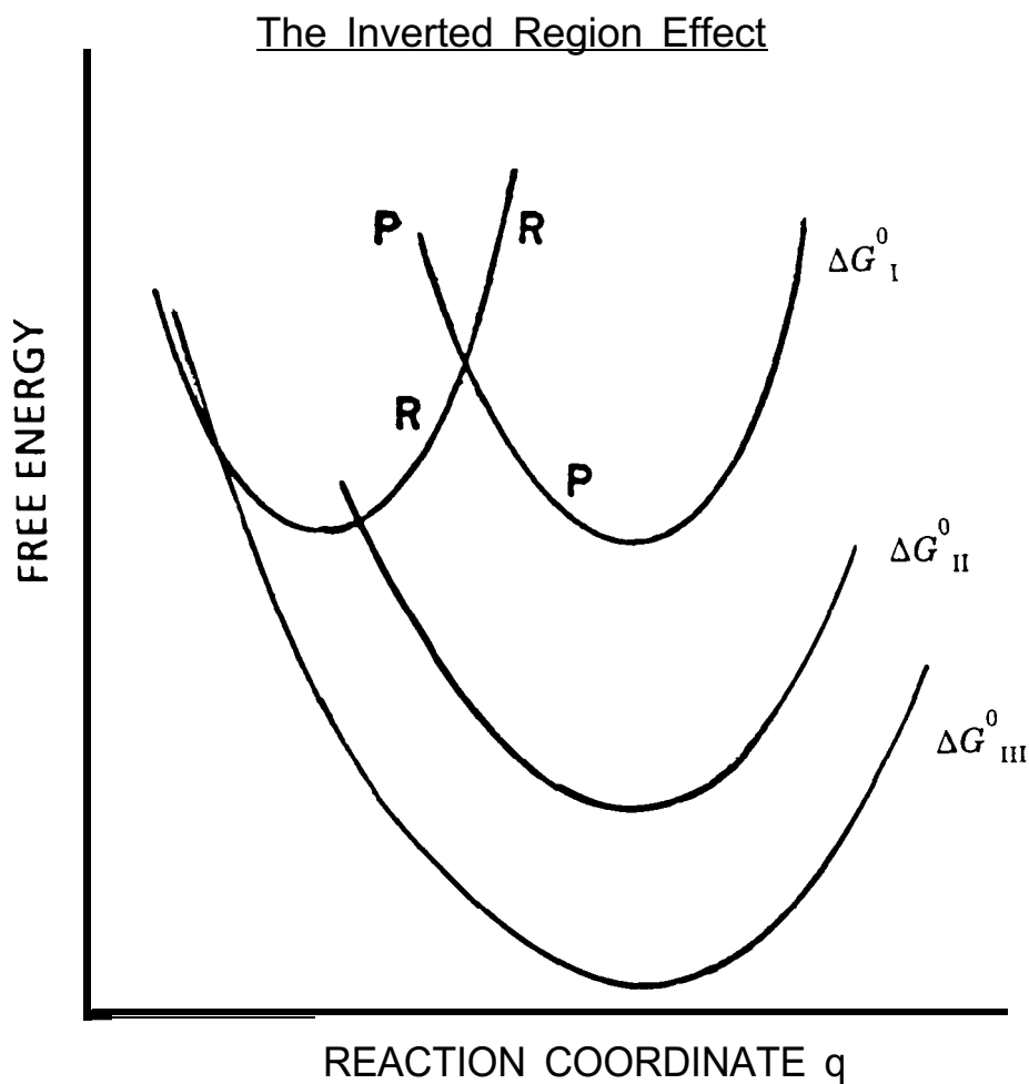
Figure 6. Plot of the free energy G versus the reaction coordinate q , for reactants' (R) and products' (P), for three different values of \Delta G^\circ , the cases I to III indicated in Figure 7 (Marcus and Siddarth, ref. 2).
