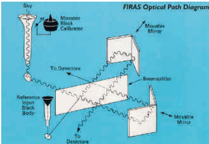
Figure 3. Concept for the Far Infrared Absolute Spectrophotometer. The movable black calibrator emits the same spectrum of radiation that is received from the sky.
