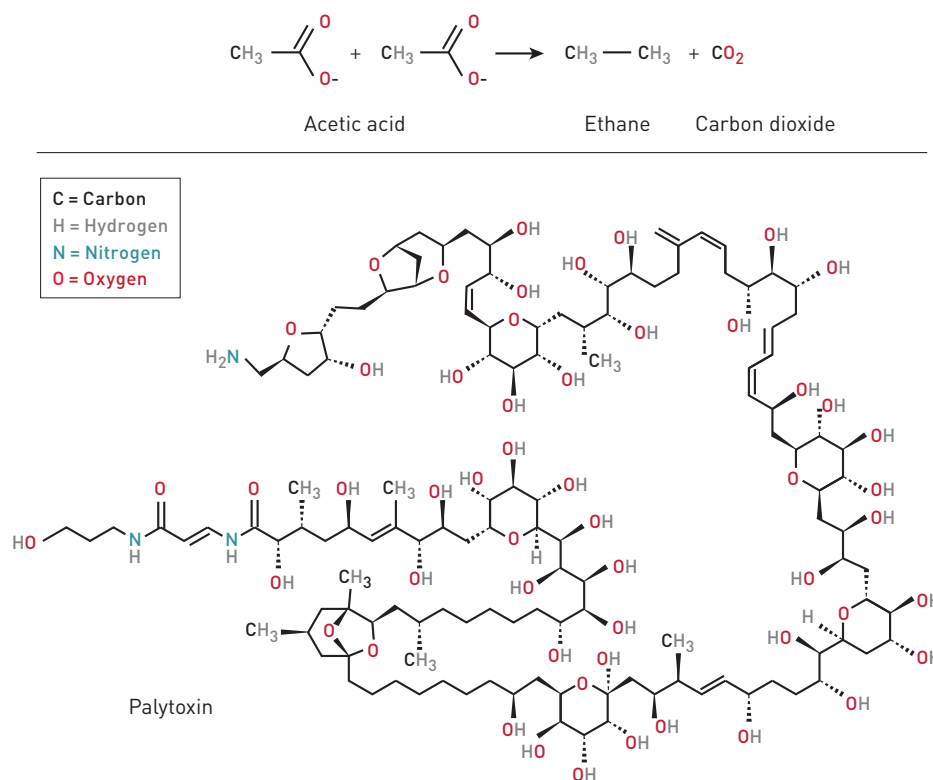
Figure 3. Organic chemistry began to develop in the middle of the nineteenth century. In one of the first reactions, the German chemist Hermann Kolbe obtained the simple molecule ethane ( \text{C}_2\text{H}_6 ) from acetic acid (top). About 150 years later, scientists were able to create palytoxin, one of the world's most complex molecules. In order to keep illustrations simple, scientists do not depict all the carbon and hydrogen atoms. In the illustration every intersection represents a carbon atom. Palytoxin consists of 129 carbon atoms, 223 hydrogen atoms, three nitrogen atoms, and 54 oxygen atoms.
