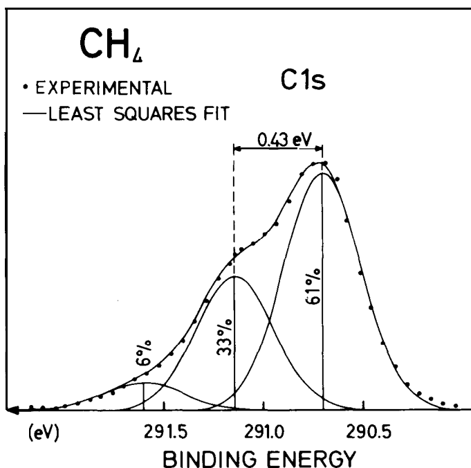
Fig. 15. Vibrational structure of the core electron line (C1s) in \text{CH}_4 . The line structure can be quantitatively explained as a consequence of the shrinkage of the equilibrium distances upon core electron mission [217].
