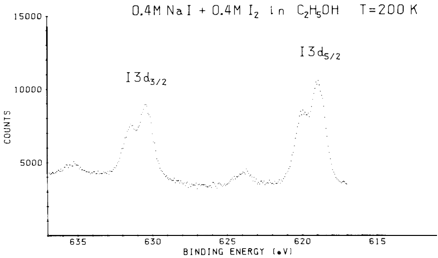
Fig. 12. I 3d spectrum from a solution of NaI (0.4M)+I 2 (0.4M) in ethanol obtained at T = 200K. The doublet for each spin-orbit component is due to ionization of the central atom (lower peak) and outer atoms (higher peak) of the I 3 ion. The extra peaks at the high-binding-energy sides of each spin-orbit component are interpreted as shake-up structures.
