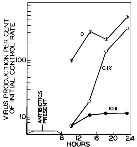
Figure 3. Effects of actinomycin D on production of Rous sarcoma virus. Chicken cells producing RSV were exposed to 0, 0.1 or 10 \mu\text{g} ( \gamma )/ml of actinomycin D. After 8 hours, the medium was removed, the cells were washed, and fresh medium was added. At the indicated times, the medium was harvested and assayed for focus forming units of RSV. (Taken from Temin, 1963.)
