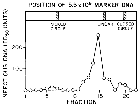
Figure 10. Electrophoresis of unintegrated infectious SNV DNA. The supernatant fraction from Hirt extraction of cells 65 hours after infection by SNV was electrophoresed in a 0.7% agarose gel in the presence of ethidium bromide with DNA from plasmid RSF 1010 as a marker. The positions of the marker DNAs were established visually, and each fraction was assayed for infectivity. (Taken from Fritsch and Temin, 1976.)
