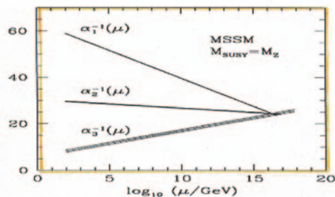
Figure 10: We can test the hypothesis that the disparate coupling strengths of the different gauge interactions derive a common value at short distances, by doing calculations to take into account the effect of virtual particle clouds [16]. These are the same sort of calculations that go into Figure 3, but extrapolated to much higher energies, or equivalently shorter distances. Top panel: using known virtual particles. Bottom panel: including also the virtual particles required by low-energy supersymmetry [17].
