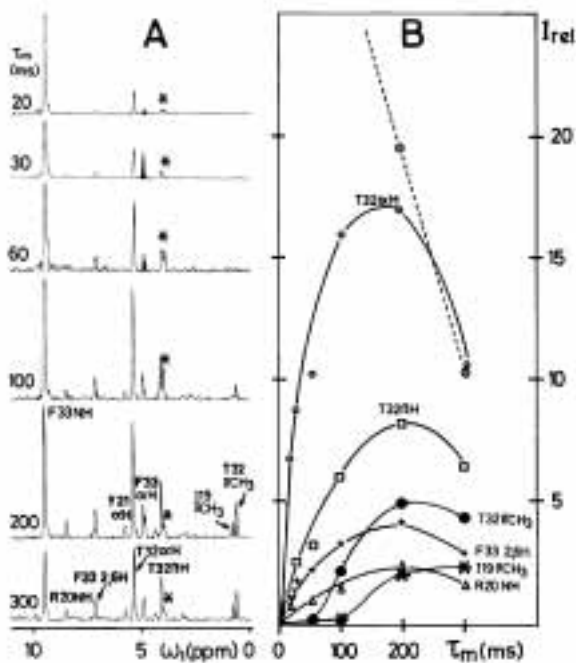
Figure 20. Measurement of NOE build-up curves using 2D [ ^1\text{H} , ^1\text{H} ]-NOESY experiments. (A) Six NOESY spectra of BPTI recorded with different mixing times, as indicated on the left. The same 1D cross-section along the \omega_1 frequency axis through the diagonal peak of the Phe 33 amide proton is plotted for each spectrum. (B) NOE build-up curves obtained from the analysis of the data in (A); same presentation as in Figure 13, with the relative intensities of the NOESY cross peaks plotted versus the length of the mixing time, \tau_m , and the broken line representing the decay of the magnetization on the diagonal peak of the Phe 33 amide proton.
