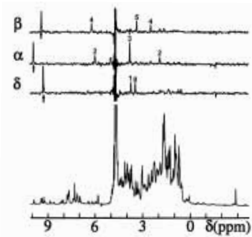
Figure 15. ^1\text{H} NMR assignments for the heme group of a c-type cytochrome using ^1\text{H} - ^{13}\text{N} NOEs (see Figure 7). Bottom trace: 1D ^1\text{H} NMR spectrum of ferrocycytochrome c-551 from Pseudomonas aeruginosa ( M \approx 12000 ). Upper traces: three 1D truncated-driven NOE difference spectra obtained with selective pre-irradiation (indicated by arrows) on the hydrogen atoms \beta , \alpha and \delta (see Figure 9), respectively (360 MHz, 35^\circ\text{C} , ^2\text{H}_2\text{O} -solution). The NOE peaks are identified with numbers indicating the substituents attached to the corresponding porphyrin ring carbons (Figure 9).
