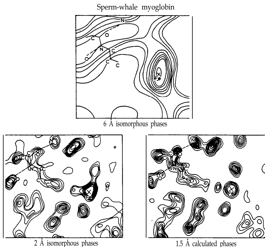
Fig. 8. Comparison between the same section through the myoglobin molecule, (i) at 6Å resolution, (ii) at 2Å resolution, (iii) at 1.4 Å resolution. ( Top left ) longitudinal section through a helix; ( right centre ) haem group edge-on. The atoms marked are part of the distal histidine (see text); note that several neighbouring atoms are resolved at 1.4Å
