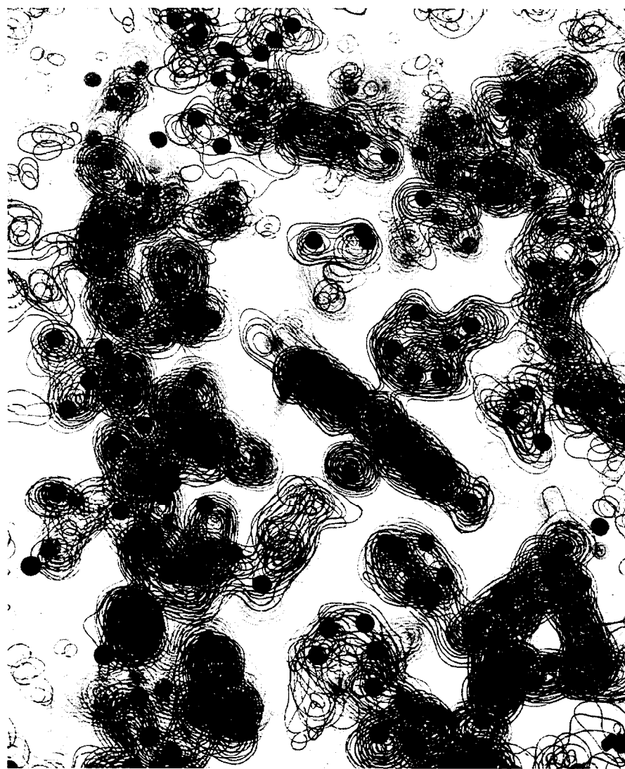
Fig.10. Part of the 1.4Å Fourier synthesis. ( Centre ) the haem group (edge-on), showing haem-linked and distal histidines, and water molecule attached to iron atom. ( Top right ) a helix end-on. ( Bottom ) a helix seen longitudinally, together with several side chains.
